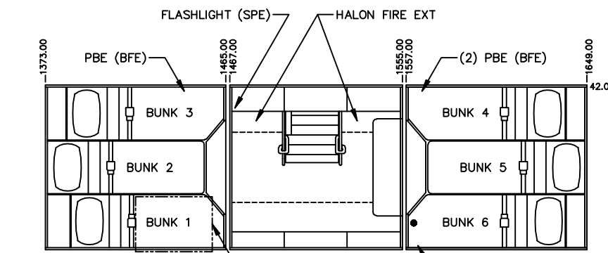
OVERHEAD FLIGHT ATTENDANT REST (OFAR) WITH SIX (6) BUNKS (SEE SHEET 3)
