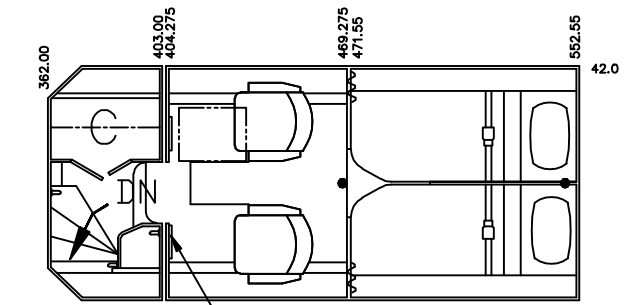
OVERHEAD FLIGHT CREW REST (OFAR) WITH TWO (2) BUNKS AND TWO(2) SEATS LITERATURE POCKET (2 PL)
